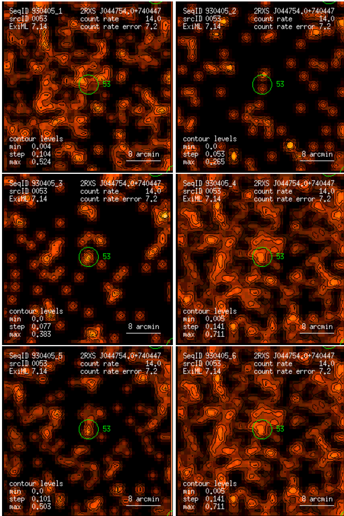
Figure 53: RASS 930405: detection 0053: band rate images, Gaussian filter: (1) PSPC channels 11 – 41, (2) 52 – 90, (3) 91 – 201, (4) 11 – 235, (5) 52 – 201, (6) 11 – 201. Broad band rates in counts/ks. Band rate contour levels in counts/ks/arcmin 2 .
