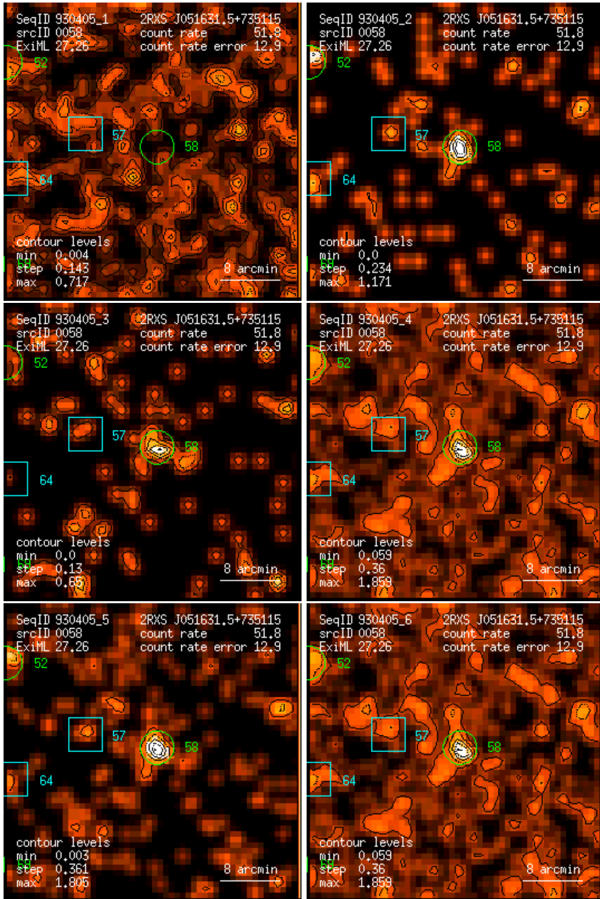
Figure 58: RASS 930405: detection 0058: band rate images, Gaussian filter: (1) PSPC channels 11 – 41, (2) 52 – 90, (3) 91 – 201, (4) 11 – 235, (5) 52 – 201, (6) 11 – 201. Broad band rates in counts/ks. Band rate contour levels in counts/ks/arcmin 2 .
