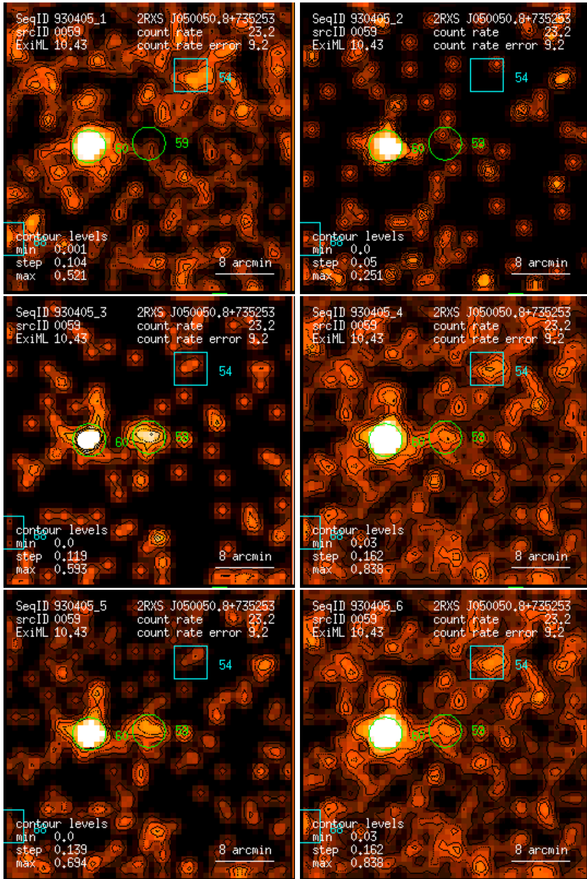
Figure 59: RASS 930405: detection 0059: band rate images, Gaussian filter: (1) PSPC channels 11 – 41, (2) 52 – 90, (3) 91 – 201, (4) 11 – 235, (5) 52 – 201, (6) 11 – 201. Broad band rates in counts/ks. Band rate contour levels in counts/ks/arcmin 2 .
