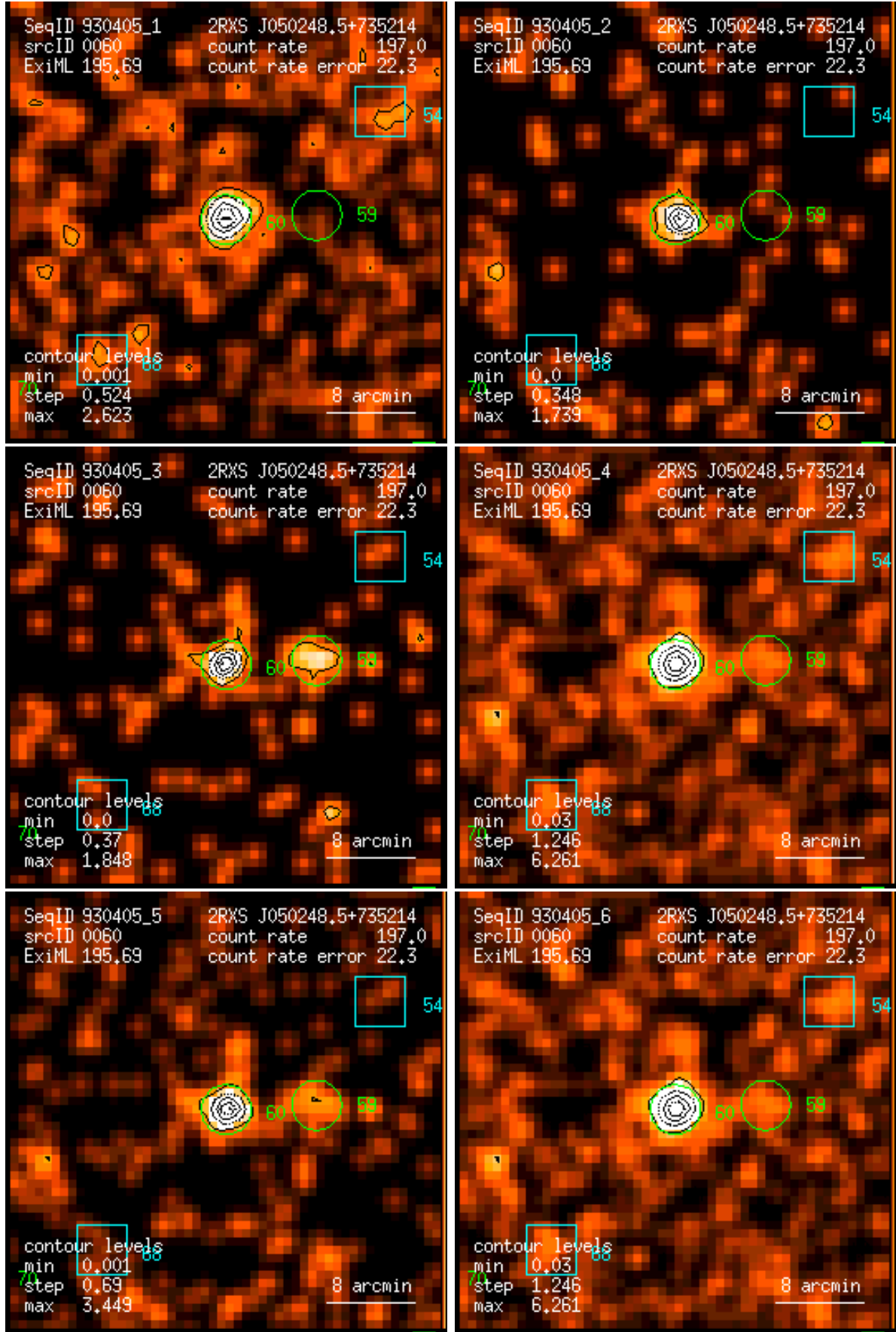
Figure 60: RASS 930405: detection 0060: band rate images, Gaussian filter: (1) PSPC channels 11 – 41, (2) 52 – 90, (3) 91 – 201, (4) 11 – 235, (5) 52 – 201, (6) 11 – 201. Broad band rates in counts/ks. Band rate contour levels in counts/ks/arcmin 2 .
