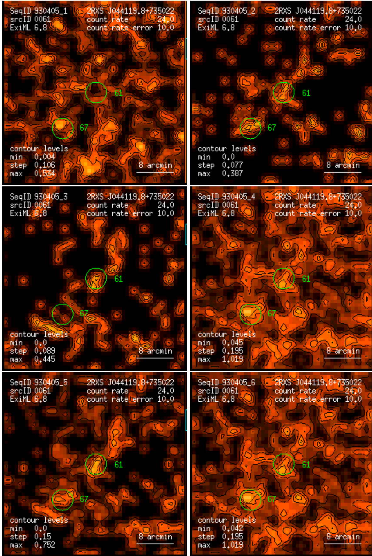
Figure 61: RASS 930405: detection 0061: band rate images, Gaussian filter: (1) PSPC channels 11 – 41, (2) 52 – 90, (3) 91 – 201, (4) 11 – 235, (5) 52 – 201, (6) 11 – 201. Broad band rates in counts/ks. Band rate contour levels in counts/ks/arcmin 2 .
