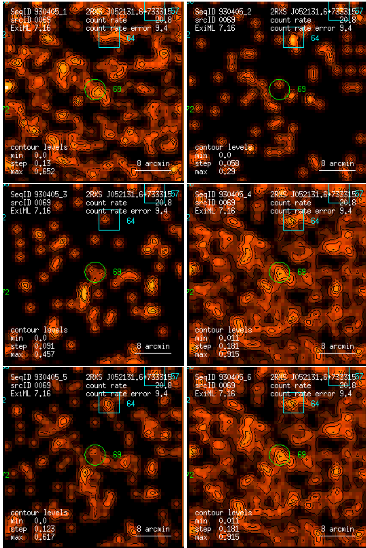
Figure 69: RASS 930405: detection 0069: band rate images, Gaussian filter: (1) PSPC channels 11 – 41, (2) 52 – 90, (3) 91 – 201, (4) 11 – 235, (5) 52 – 201, (6) 11 – 201. Broad band rates in counts/ks. Band rate contour levels in counts/ks/arcmin 2 .
