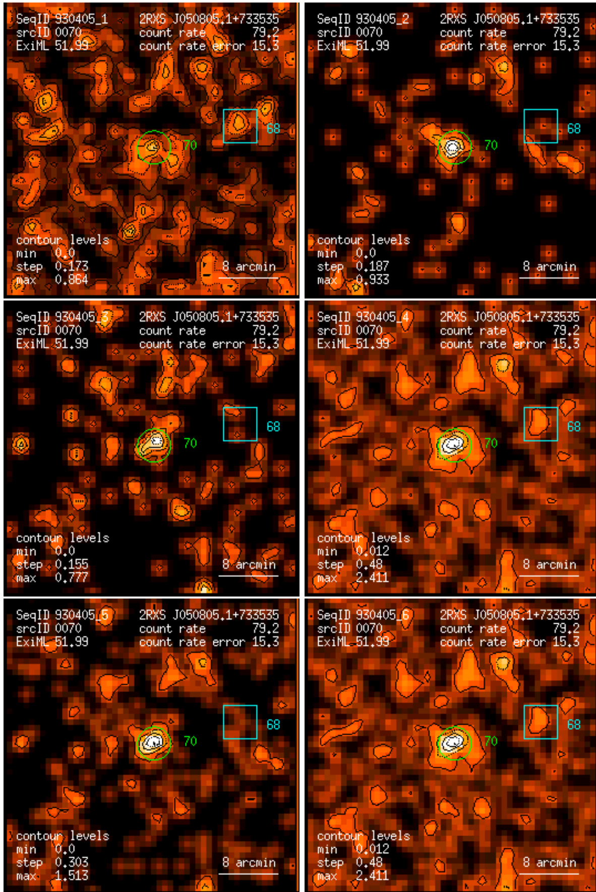
Figure 70: RASS 930405: detection 0070: band rate images, Gaussian filter: (1) PSPC channels 11 – 41, (2) 52 – 90, (3) 91 – 201, (4) 11 – 235, (5) 52 – 201, (6) 11 – 201. Broad band rates in counts/ks. Band rate contour levels in counts/ks/arcmin 2 .
