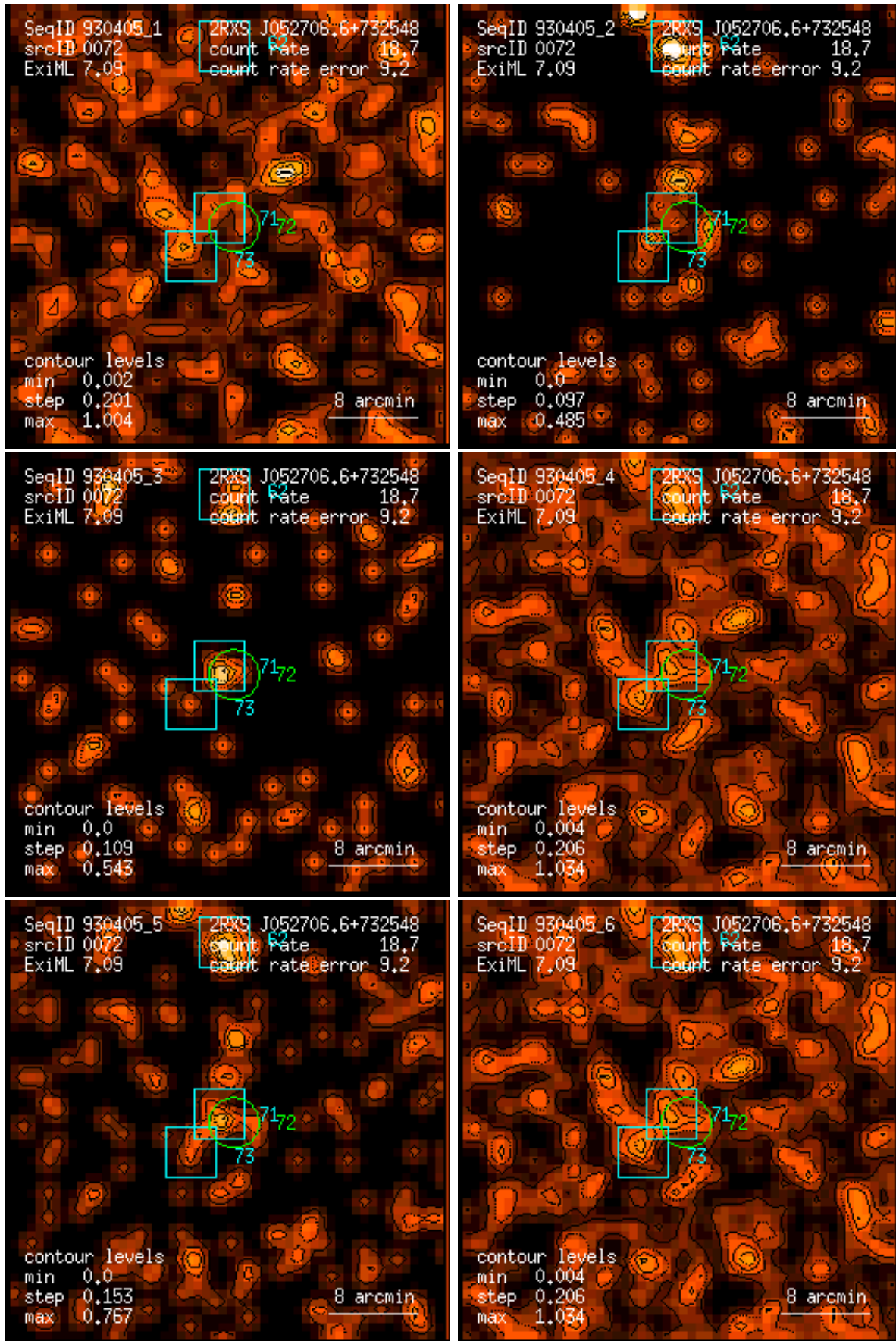
Figure 72: RASS 930405: detection 0072: band rate images, Gaussian filter: (1) PSPC channels 11 – 41, (2) 52 – 90, (3) 91 – 201, (4) 11 – 235, (5) 52 – 201, (6) 11 – 201. Broad band rates in counts/ks. Band rate contour levels in counts/ks/arcmin 2 .
