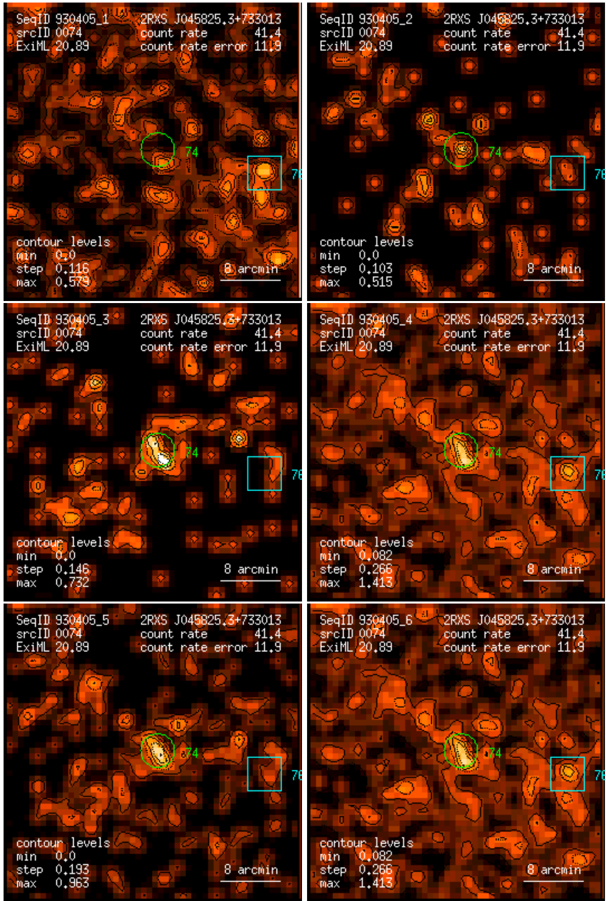
Figure 74: RASS 930405: detection 0074: band rate images, Gaussian filter: (1) PSPC channels 11 – 41, (2) 52 – 90, (3) 91 – 201, (4) 11 – 235, (5) 52 – 201, (6) 11 – 201. Broad band rates in counts/ks. Band rate contour levels in counts/ks/arcmin 2 .
