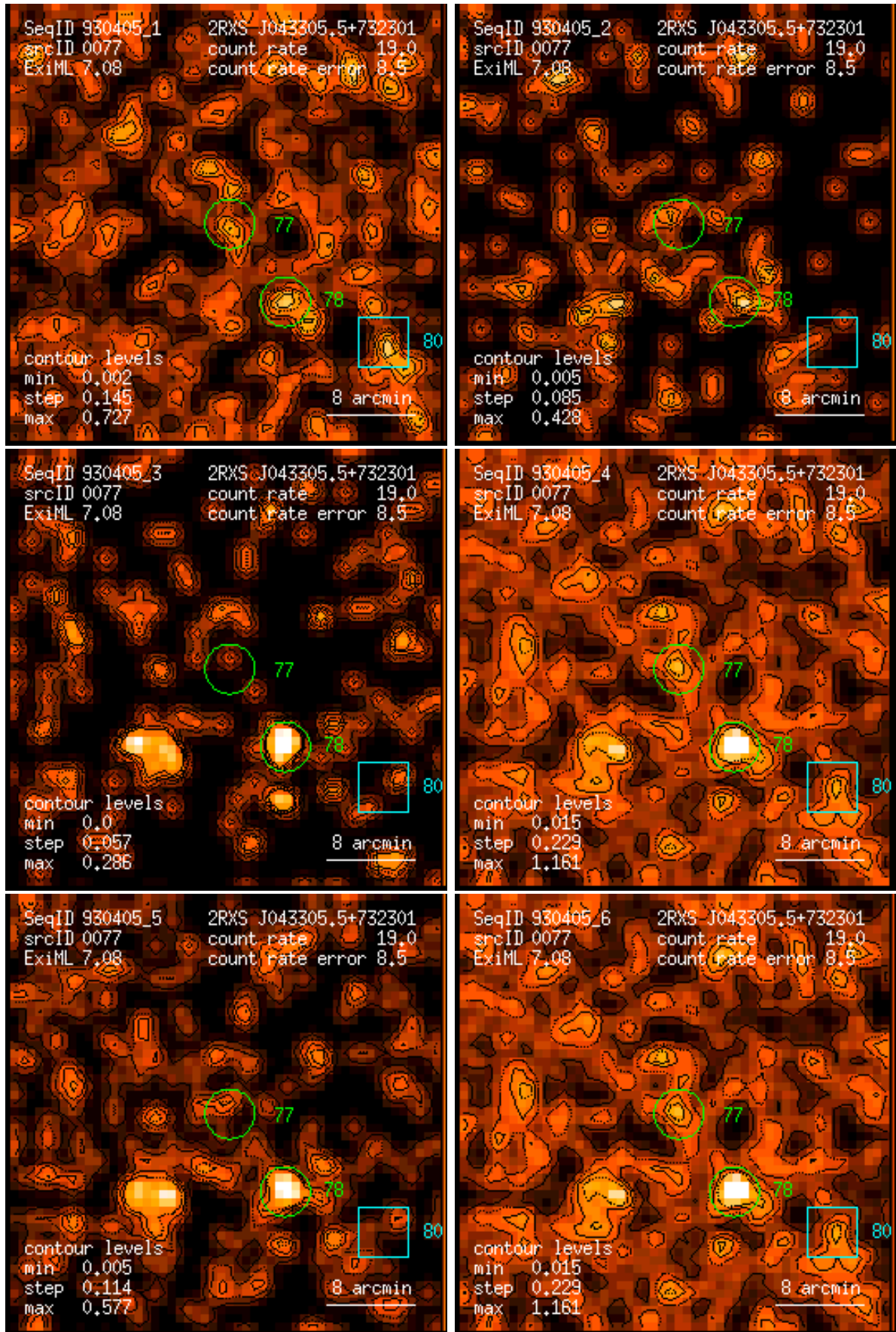
Figure 77: RASS 930405: detection 0077: band rate images, Gaussian filter: (1) PSPC channels 11 – 41, (2) 52 – 90, (3) 91 – 201, (4) 11 – 235, (5) 52 – 201, (6) 11 – 201. Broad band rates in counts/ks. Band rate contour levels in counts/ks/arcmin 2 .
