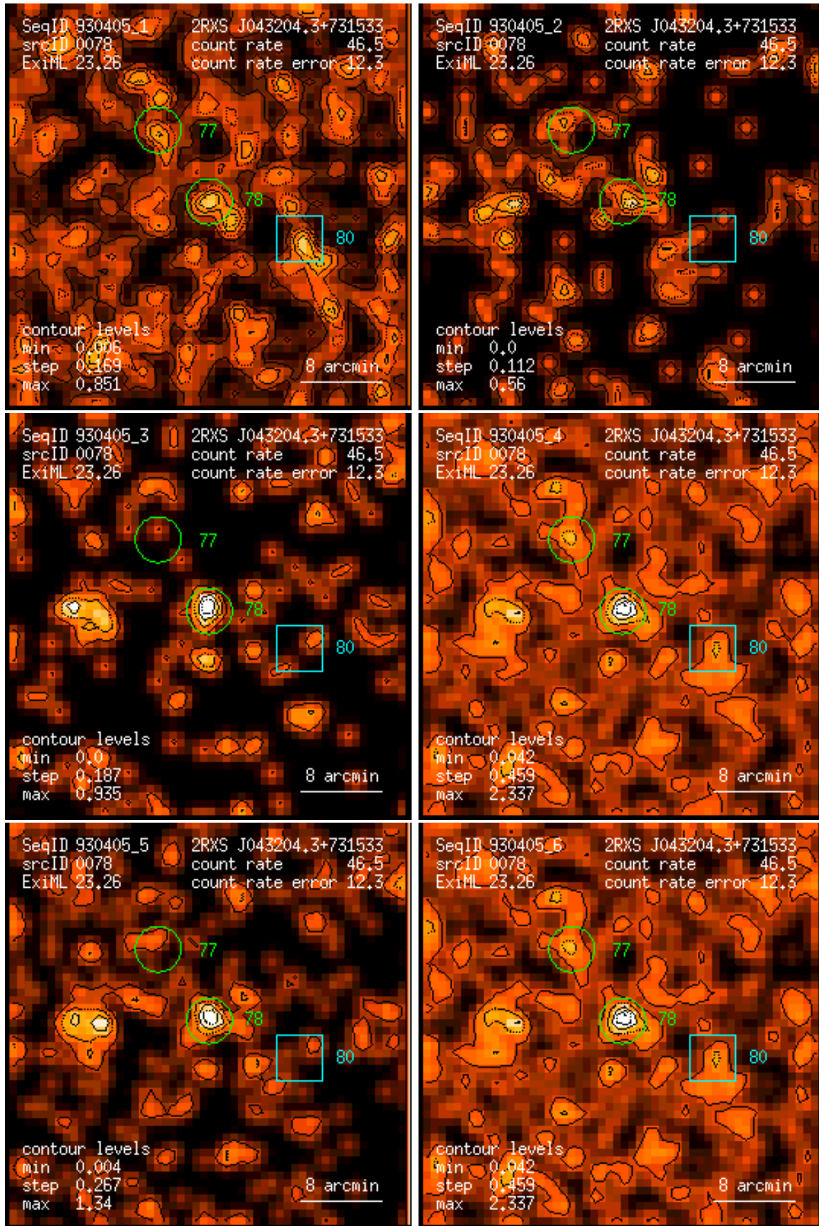
Figure 78: RASS 930405: detection 0078: band rate images, Gaussian filter: (1) PSPC channels 11 – 41, (2) 52 – 90, (3) 91 – 201, (4) 11 – 235, (5) 52 – 201, (6) 11 – 201. Broad band rates in counts/ks. Band rate contour levels in counts/ks/arcmin 2 .
