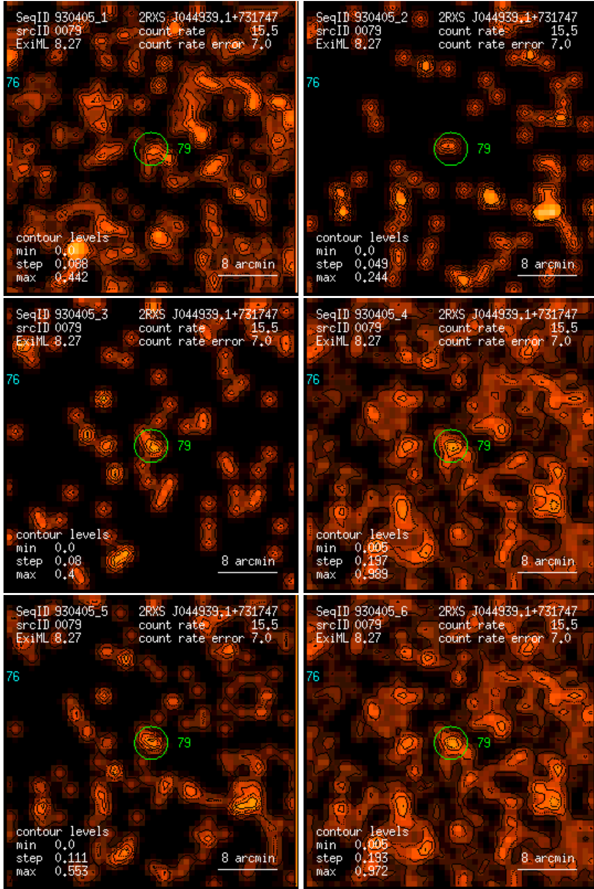
Figure 79: RASS 930405: detection 0079: band rate images, Gaussian filter: (1) PSPC channels 11 – 41, (2) 52 – 90, (3) 91 – 201, (4) 11 – 235, (5) 52 – 201, (6) 11 – 201. Broad band rates in counts/ks. Band rate contour levels in counts/ks/arcmin 2 .
