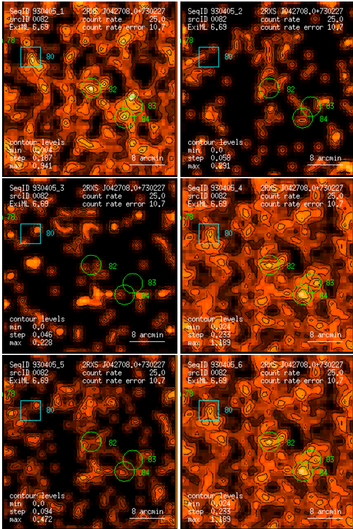
Figure 82: RASS 930405: detection 0082: band rate images, Gaussian filter: (1) PSPC channels 11 – 41, (2) 52 – 90, (3) 91 – 201, (4) 11 – 235, (5) 52 – 201, (6) 11 – 201. Broad band rates in counts/ks. Band rate contour levels in counts/ks/arcmin 2 .
