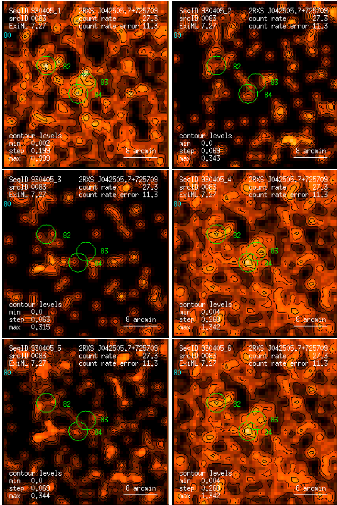
Figure 83: RASS 930405: detection 0083: band rate images, Gaussian filter: (1) PSPC channels 11 – 41, (2) 52 – 90, (3) 91 – 201, (4) 11 – 235, (5) 52 – 201, (6) 11 – 201. Broad band rates in counts/ks. Band rate contour levels in counts/ks/arcmin 2 .
