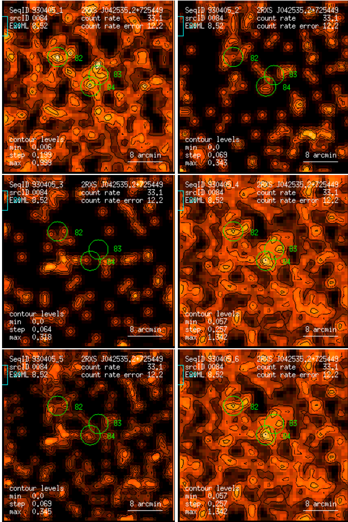
Figure 84: RASS 930405: detection 0084: band rate images, Gaussian filter: (1) PSPC channels 11 – 41, (2) 52 – 90, (3) 91 – 201, (4) 11 – 235, (5) 52 – 201, (6) 11 – 201. Broad band rates in counts/ks. Band rate contour levels in counts/ks/arcmin 2 .
