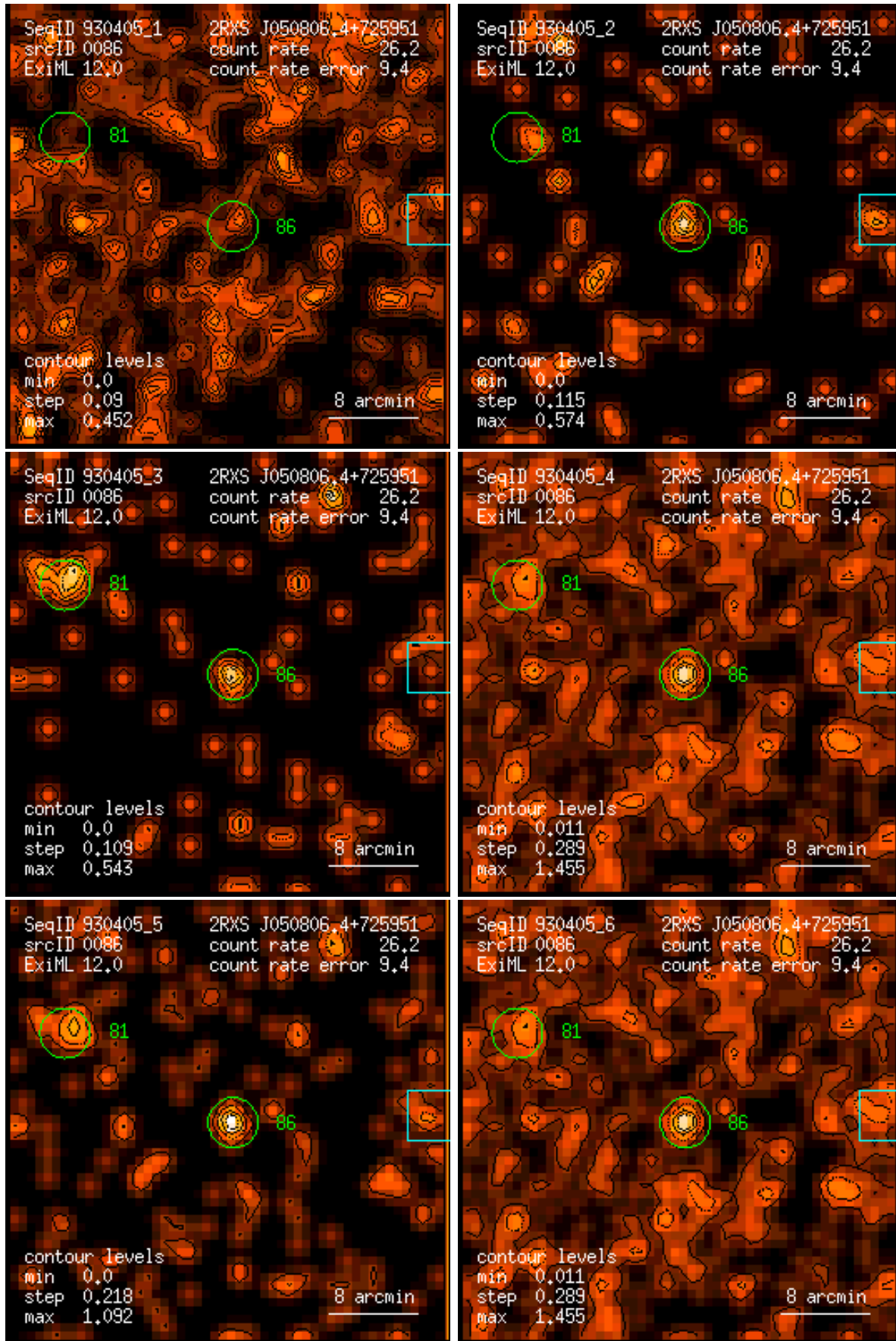
Figure 86: RASS 930405: detection 0086: band rate images, Gaussian filter: (1) PSPC channels 11 – 41, (2) 52 – 90, (3) 91 – 201, (4) 11 – 235, (5) 52 – 201, (6) 11 – 201. Broad band rates in counts/ks. Band rate contour levels in counts/ks/arcmin 2 .
