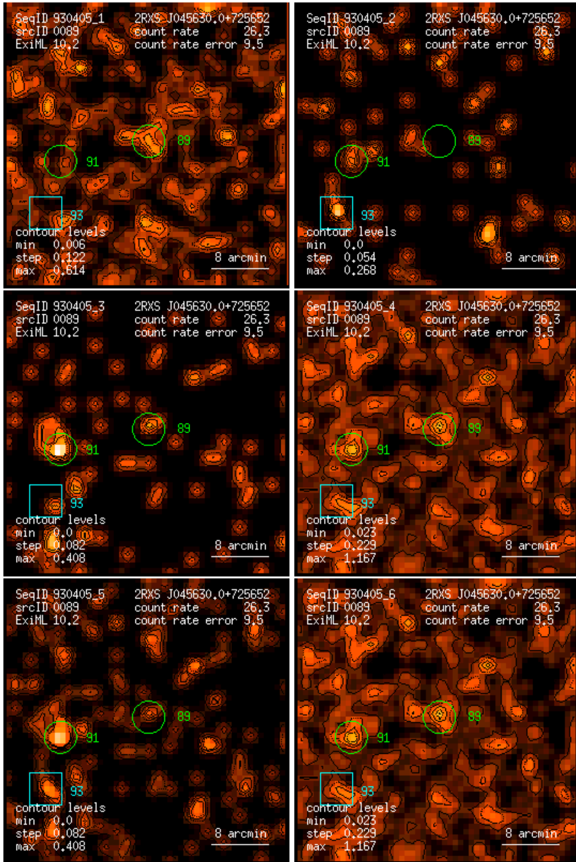
Figure 89: RASS 930405: detection 0089: band rate images, Gaussian filter: (1) PSPC channels 11 – 41, (2) 52 – 90, (3) 91 – 201, (4) 11 – 235, (5) 52 – 201, (6) 11 – 201. Broad band rates in counts/ks. Band rate contour levels in counts/ks/arcmin 2 .
