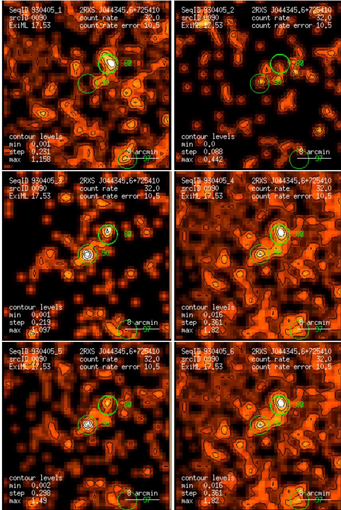
Figure 90: RASS 930405: detection 0090: band rate images, Gaussian filter: (1) PSPC channels 11 – 41, (2) 52 – 90, (3) 91 – 201, (4) 11 – 235, (5) 52 – 201, (6) 11 – 201. Broad band rates in counts/ks. Band rate contour levels in counts/ks/arcmin 2 .
