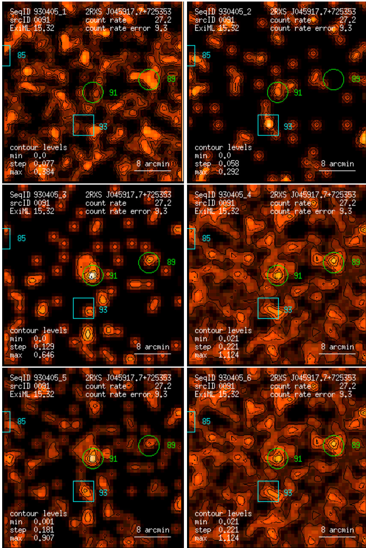
Figure 91: RASS 930405: detection 0091: band rate images, Gaussian filter: (1) PSPC channels 11 – 41, (2) 52 – 90, (3) 91 – 201, (4) 11 – 235, (5) 52 – 201, (6) 11 – 201. Broad band rates in counts/ks. Band rate contour levels in counts/ks/arcmin 2 .
