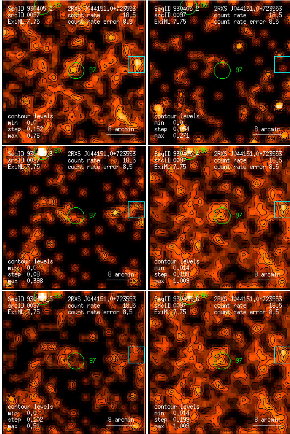
Figure 97: RASS 930405: detection 0097: band rate images, Gaussian filter: (1) PSPC channels 11 – 41, (2) 52 – 90, (3) 91 – 201, (4) 11 – 235, (5) 52 – 201, (6) 11 – 201. Broad band rates in counts/ks. Band rate contour levels in counts/ks/arcmin 2 .
