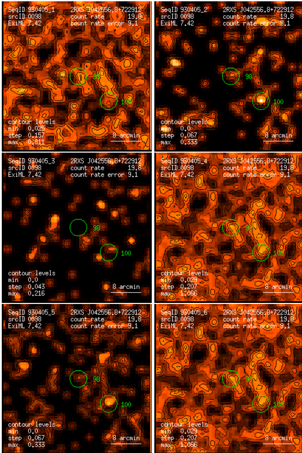
Figure 98: RASS 930405: detection 0098: band rate images, Gaussian filter: (1) PSPC channels 11 – 41, (2) 52 – 90, (3) 91 – 201, (4) 11 – 235, (5) 52 – 201, (6) 11 – 201. Broad band rates in counts/ks. Band rate contour levels in counts/ks/arcmin 2 .
