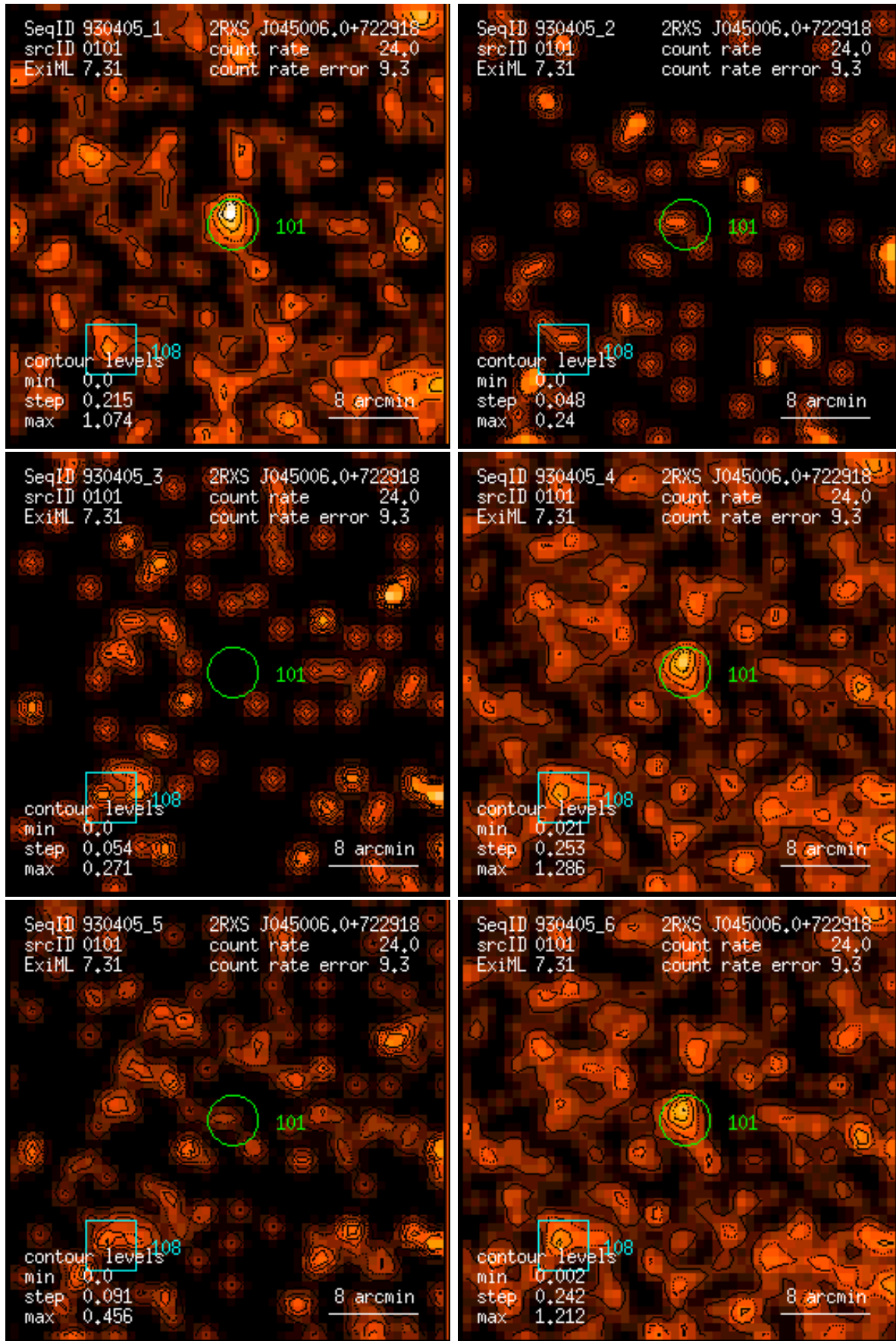
Figure 101: RASS 930405: detection 0101: band rate images, Gaussian filter: (1) PSPC channels 11 – 41, (2) 52 – 90, (3) 91 – 201, (4) 11 – 235, (5) 52 – 201, (6) 11 – 201. Broad band rates in counts/ks. Band rate contour levels in counts/ks/arcmin 2 .
