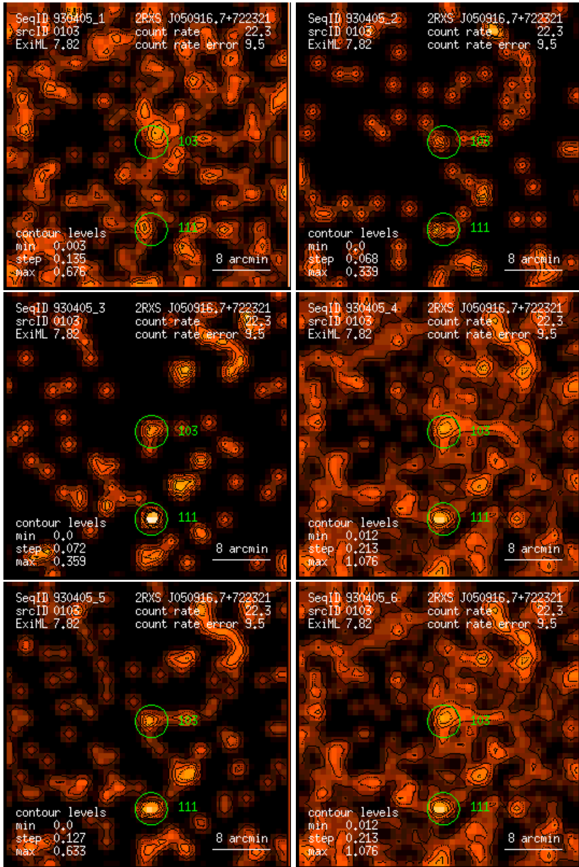
Figure 103: RASS 930405: detection 0103: band rate images, Gaussian filter: (1) PSPC channels 11 – 41, (2) 52 – 90, (3) 91 – 201, (4) 11 – 235, (5) 52 – 201, (6) 11 – 201. Broad band rates in counts/ks. Band rate contour levels in counts/ks/arcmin 2 .
