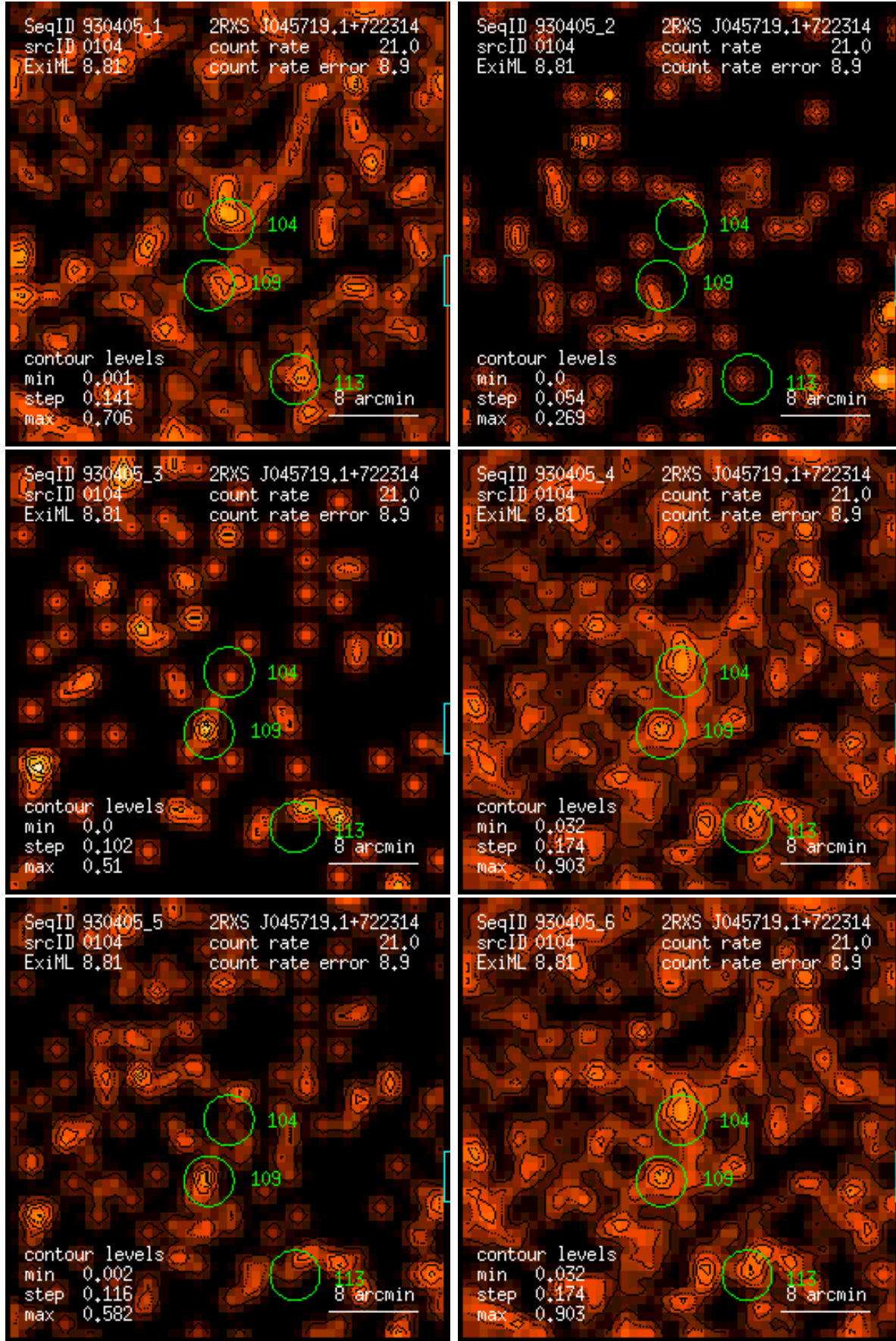
Figure 104: RASS 930405: detection 0104: band rate images, Gaussian filter: (1) PSPC channels 11 – 41, (2) 52 – 90, (3) 91 – 201, (4) 11 – 235, (5) 52 – 201, (6) 11 – 201. Broad band rates in counts/ks. Band rate contour levels in counts/ks/arcmin 2 .
