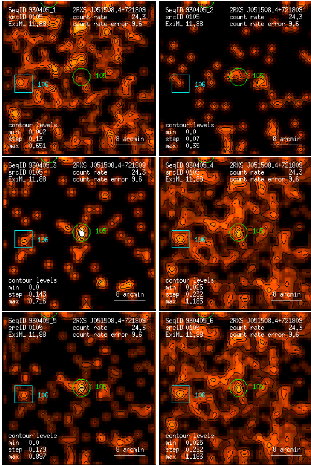
Figure 105: RASS 930405: detection 0105: band rate images, Gaussian filter: (1) PSPC channels 11 – 41, (2) 52 – 90, (3) 91 – 201, (4) 11 – 235, (5) 52 – 201, (6) 11 – 201. Broad band rates in counts/ks. Band rate contour levels in counts/ks/arcmin 2 .
