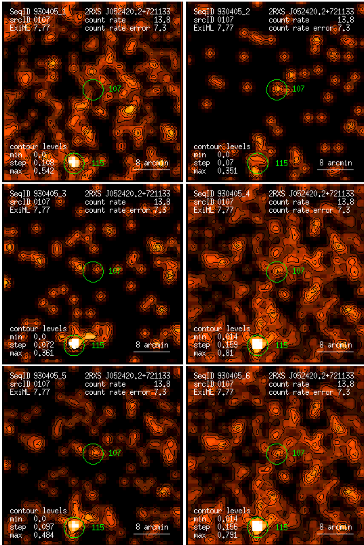
Figure 107: RASS 930405: detection 0107: band rate images, Gaussian filter: (1) PSPC channels 11 – 41, (2) 52 – 90, (3) 91 – 201, (4) 11 – 235, (5) 52 – 201, (6) 11 – 201. Broad band rates in counts/ks. Band rate contour levels in counts/ks/arcmin 2 .
