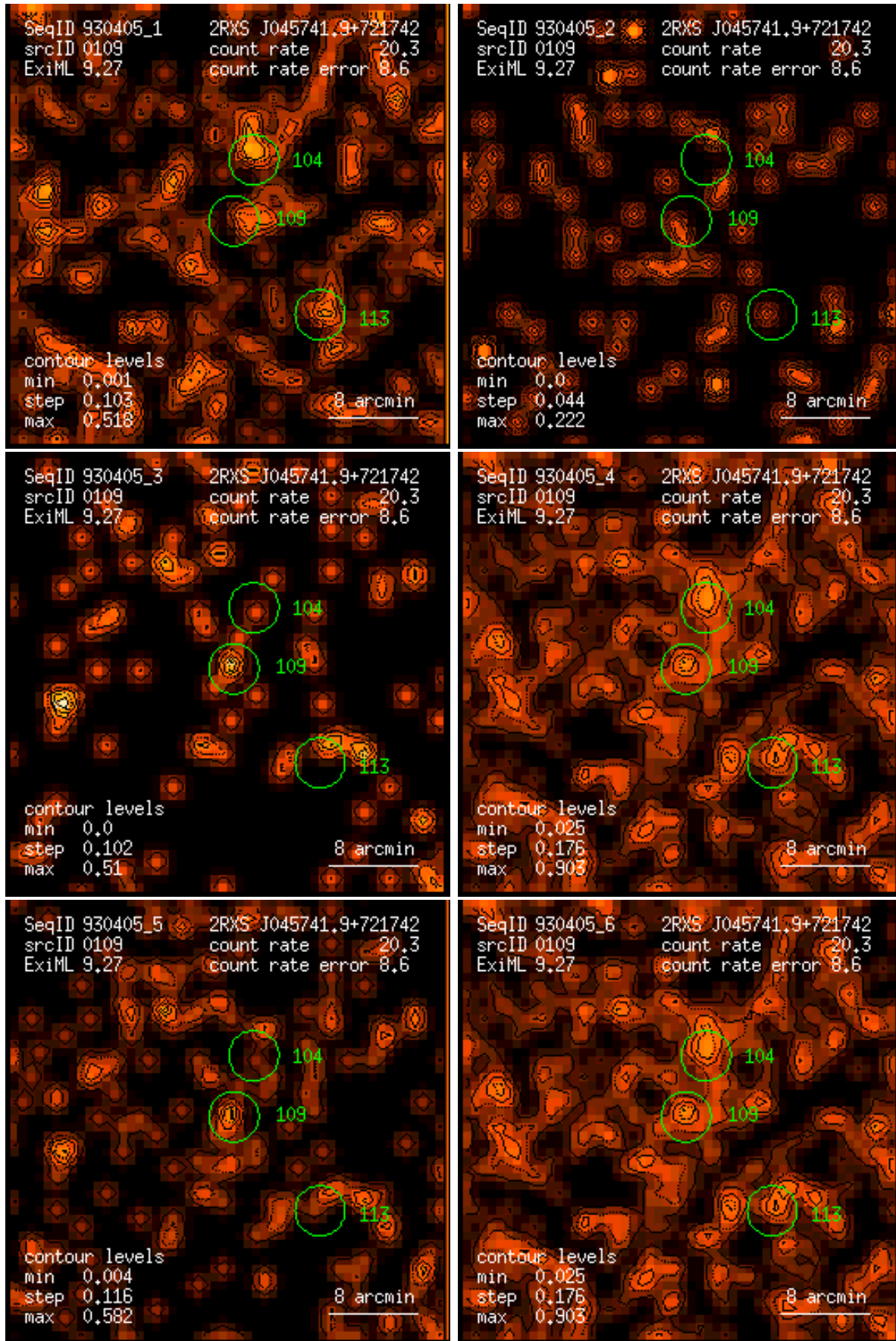
Figure 109: RASS 930405: detection 0109: band rate images, Gaussian filter: (1) PSPC channels 11 – 41, (2) 52 – 90, (3) 91 – 201, (4) 11 – 235, (5) 52 – 201, (6) 11 – 201. Broad band rates in counts/ks. Band rate contour levels in counts/ks/arcmin 2 .
