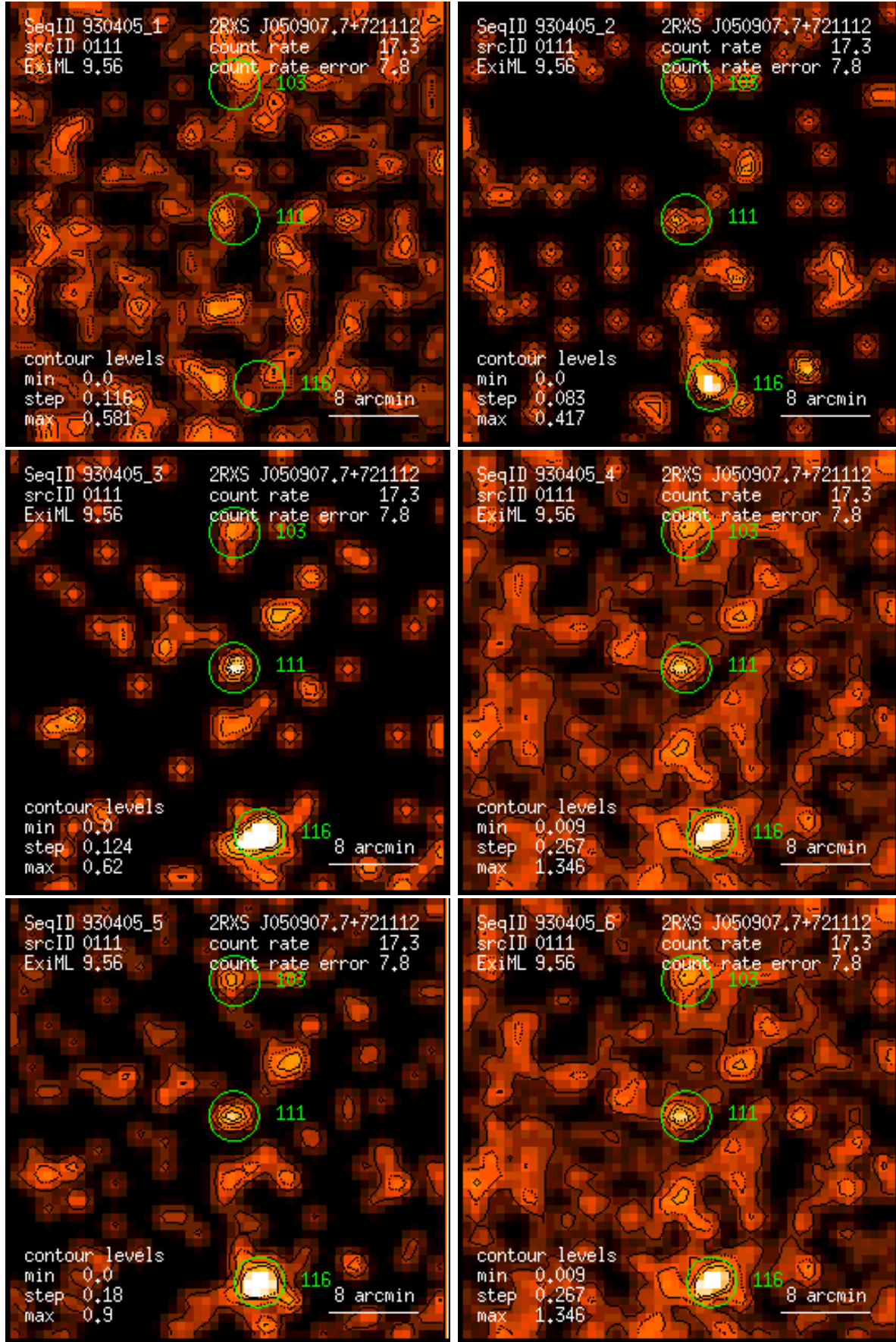
Figure 111: RASS 930405: detection 0111: band rate images, Gaussian filter: (1) PSPC channels 11 – 41, (2) 52 – 90, (3) 91 – 201, (4) 11 – 235, (5) 52 – 201, (6) 11 – 201. Broad band rates in counts/ks. Band rate contour levels in counts/ks/arcmin 2 .
