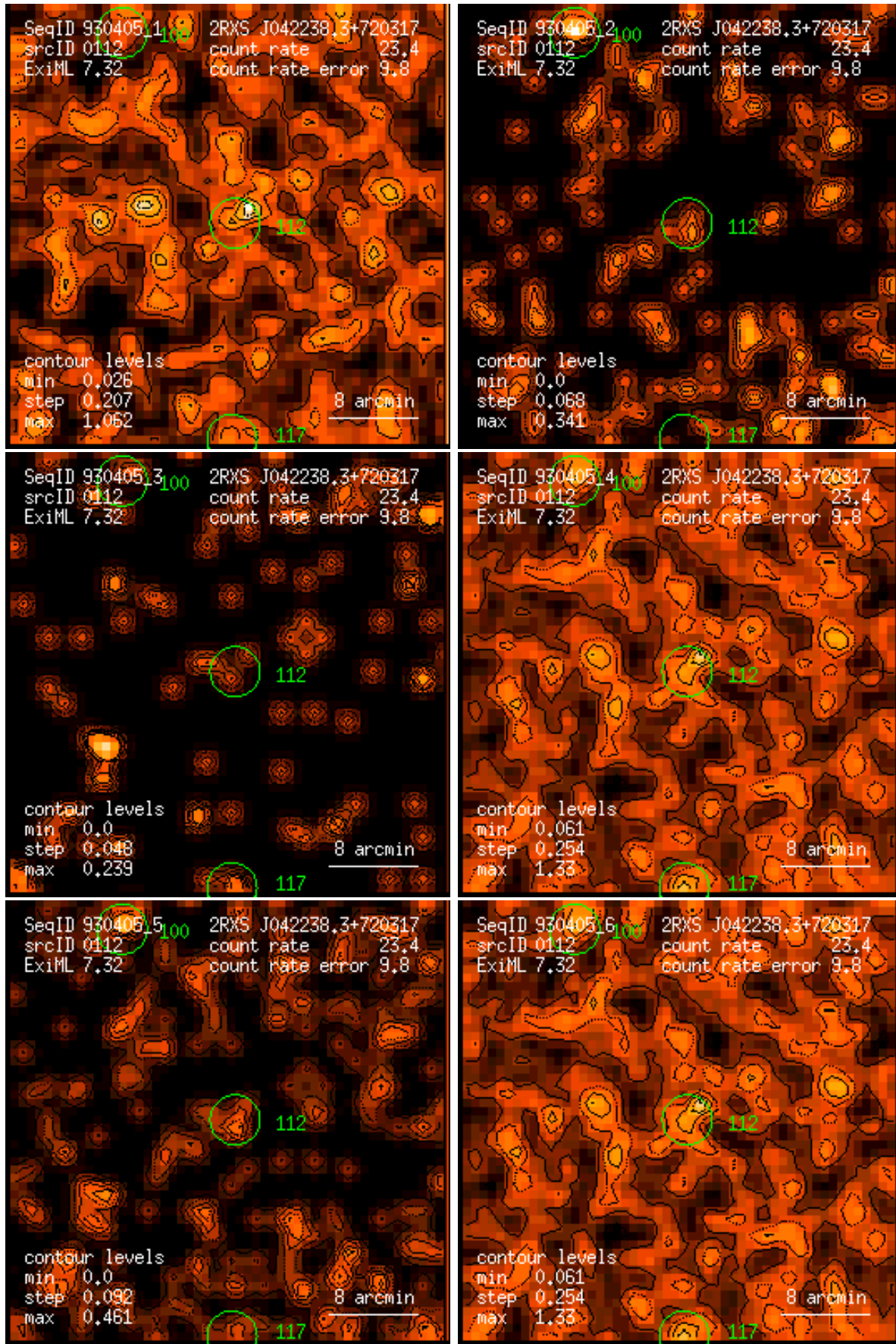
Figure 112: RASS 930405: detection 0112: band rate images, Gaussian filter: (1) PSPC channels 11 – 41, (2) 52 – 90, (3) 91 – 201, (4) 11 – 235, (5) 52 – 201, (6) 11 – 201. Broad band rates in counts/ks. Band rate contour levels in counts/ks/arcmin 2 .
