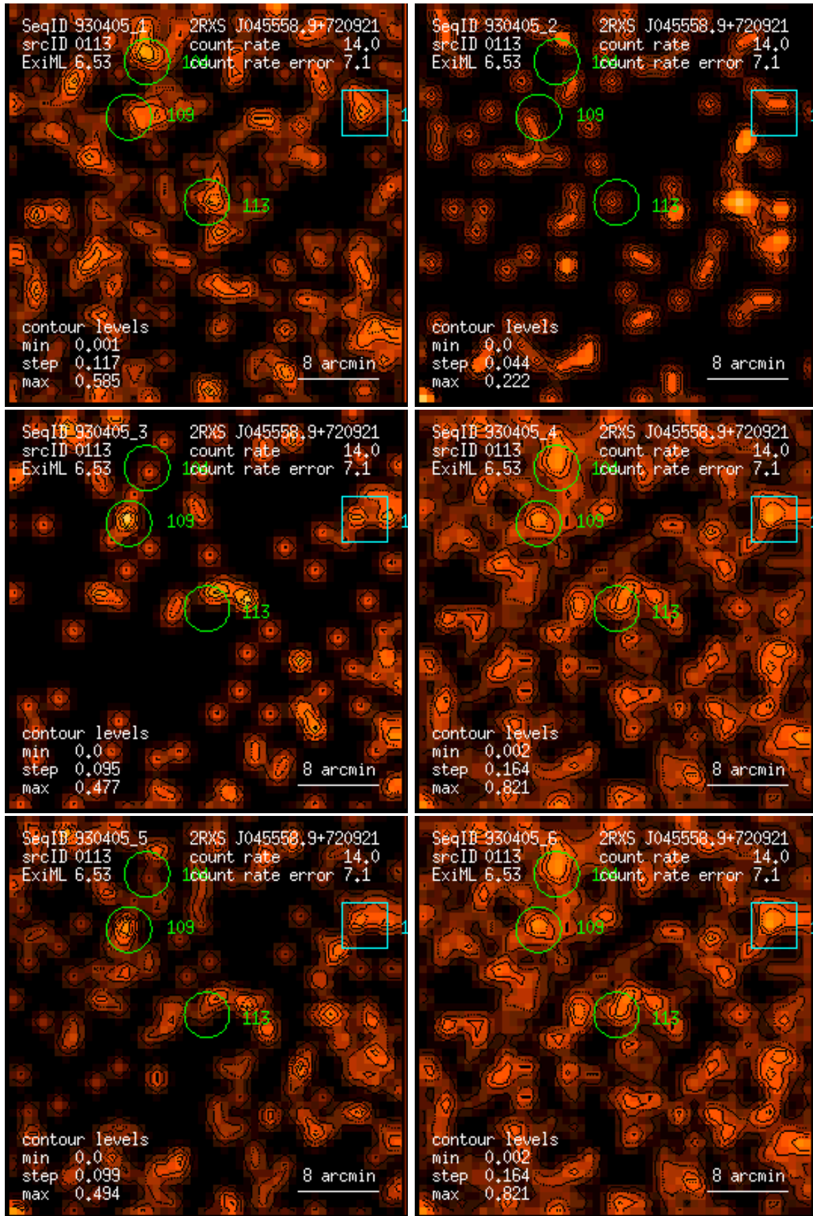
Figure 113: RASS 930405: detection 0113: band rate images, Gaussian filter: (1) PSPC channels 11 – 41, (2) 52 – 90, (3) 91 – 201, (4) 11 – 235, (5) 52 – 201, (6) 11 – 201. Broad band rates in counts/ks. Band rate contour levels in counts/ks/arcmin 2 .
