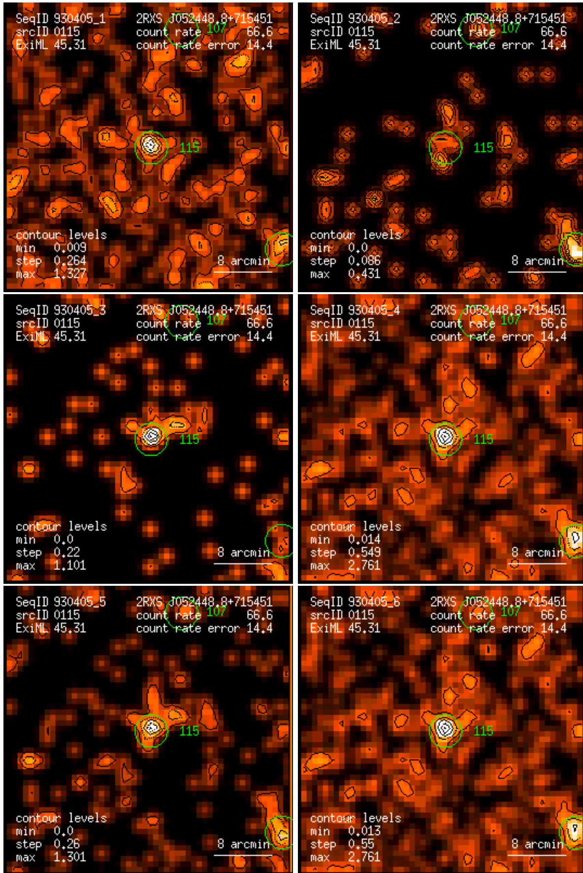
Figure 115: RASS 930405: detection 0115: band rate images, Gaussian filter: (1) PSPC channels 11 – 41, (2) 52 – 90, (3) 91 – 201, (4) 11 – 235, (5) 52 – 201, (6) 11 – 201. Broad band rates in counts/ks. Band rate contour levels in counts/ks/arcmin 2 .
