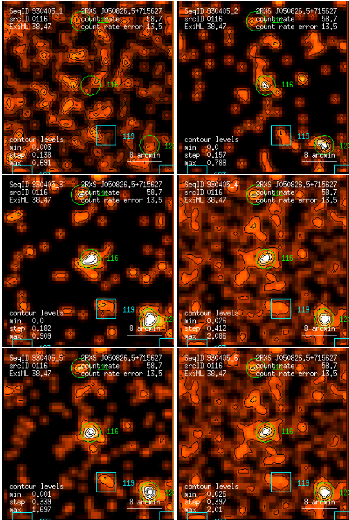
Figure 116: RASS 930405: detection 0116: band rate images, Gaussian filter: (1) PSPC channels 11 – 41, (2) 52 – 90, (3) 91 – 201, (4) 11 – 235, (5) 52 – 201, (6) 11 – 201. Broad band rates in counts/ks. Band rate contour levels in counts/ks/arcmin 2 .
