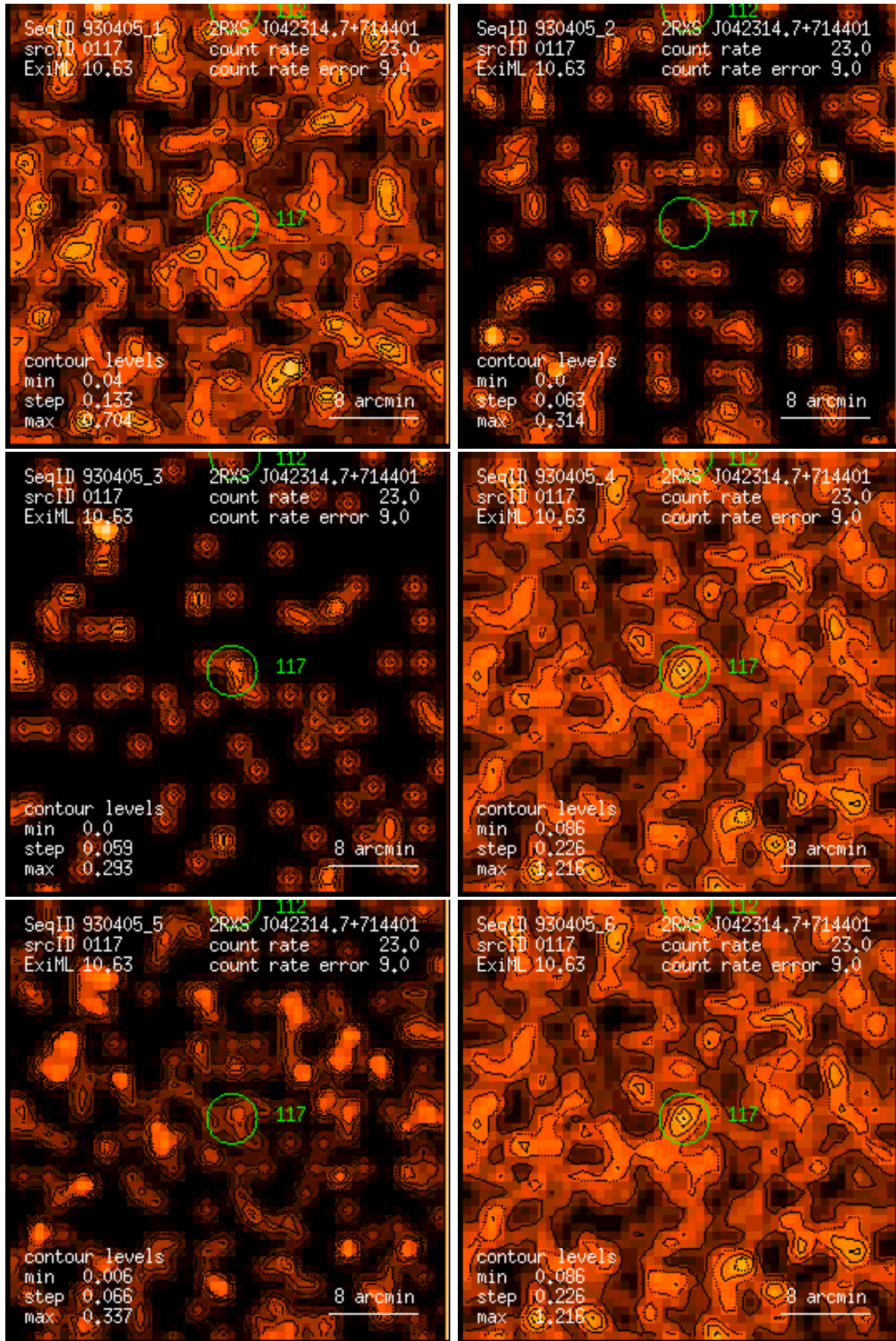
Figure 117: RASS 930405: detection 0117: band rate images, Gaussian filter: (1) PSPC channels 11 – 41, (2) 52 – 90, (3) 91 – 201, (4) 11 – 235, (5) 52 – 201, (6) 11 – 201. Broad band rates in counts/ks. Band rate contour levels in counts/ks/arcmin 2 .
