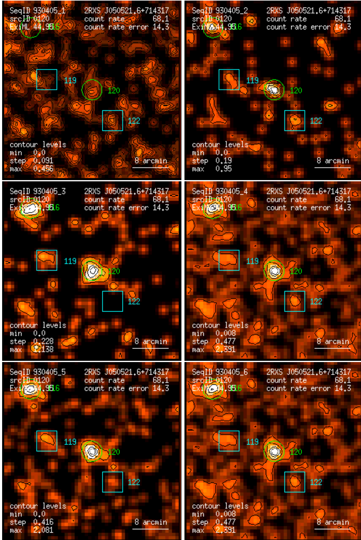
Figure 120: RASS 930405: detection 0120: band rate images, Gaussian filter: (1) PSPC channels 11 – 41, (2) 52 – 90, (3) 91 – 201, (4) 11 – 235, (5) 52 – 201, (6) 11 – 201. Broad band rates in counts/ks. Band rate contour levels in counts/ks/arcmin 2 .
