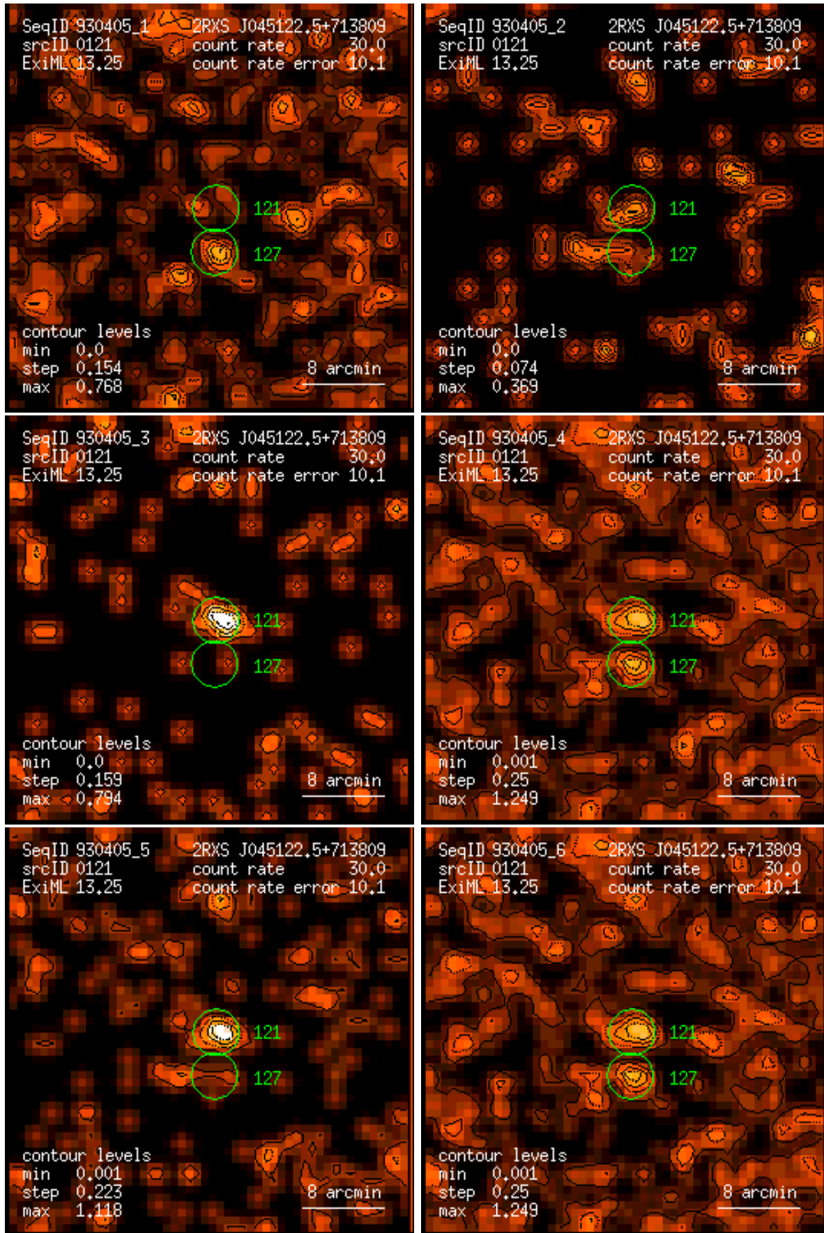
Figure 121: RASS 930405: detection 0121: band rate images, Gaussian filter: (1) PSPC channels 11 – 41, (2) 52 – 90, (3) 91 – 201, (4) 11 – 235, (5) 52 – 201, (6) 11 – 201. Broad band rates in counts/ks. Band rate contour levels in counts/ks/arcmin 2 .
