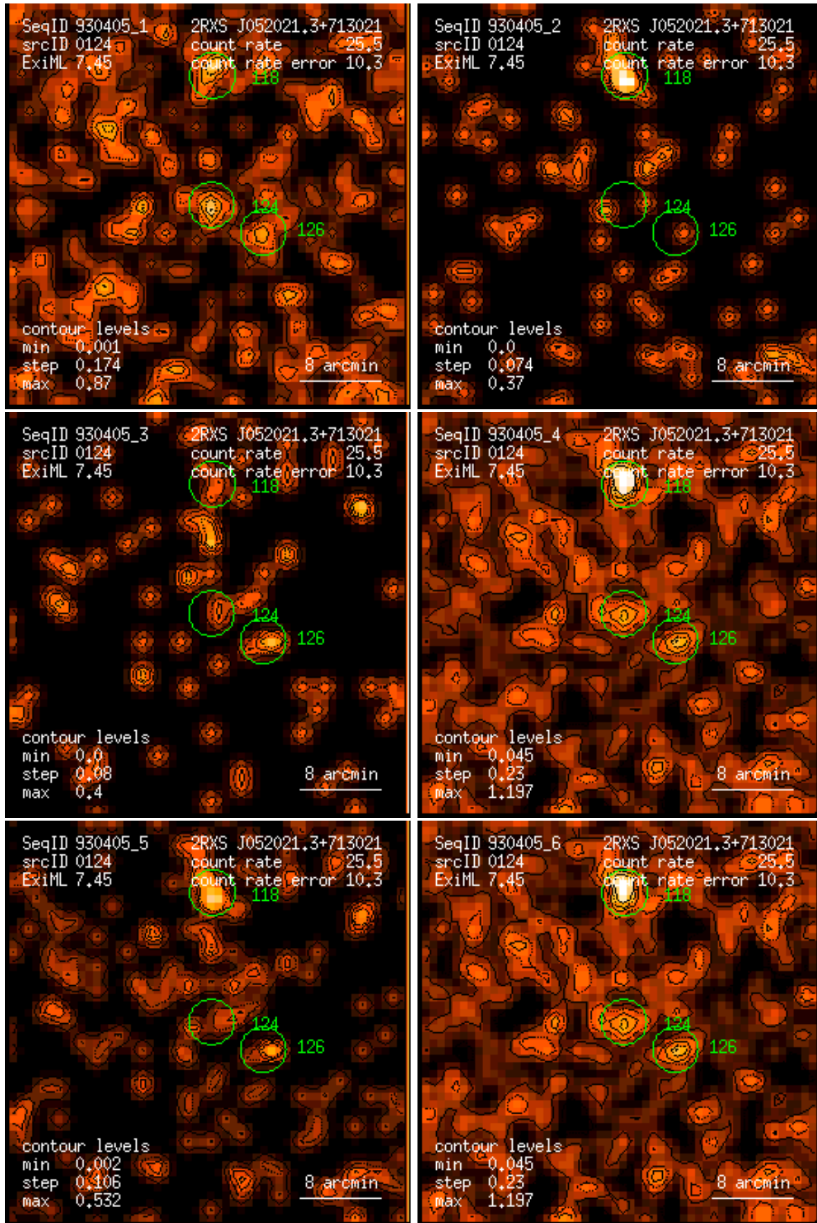
Figure 124: RASS 930405: detection 0124: band rate images, Gaussian filter: (1) PSPC channels 11 – 41, (2) 52 – 90, (3) 91 – 201, (4) 11 – 235, (5) 52 – 201, (6) 11 – 201. Broad band rates in counts/ks. Band rate contour levels in counts/ks/arcmin 2 .
