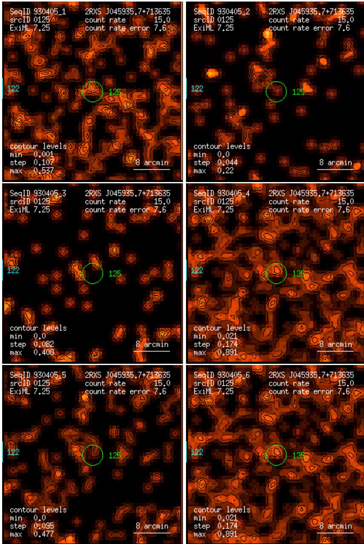
Figure 125: RASS 930405: detection 0125: band rate images, Gaussian filter: (1) PSPC channels 11 – 41, (2) 52 – 90, (3) 91 – 201, (4) 11 – 235, (5) 52 – 201, (6) 11 – 201. Broad band rates in counts/ks. Band rate contour levels in counts/ks/arcmin 2 .
