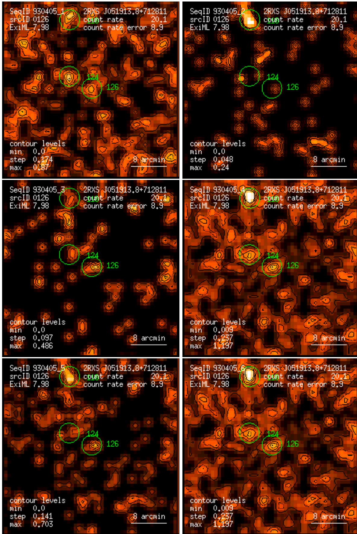
Figure 126: RASS 930405: detection 0126: band rate images, Gaussian filter: (1) PSPC channels 11 – 41, (2) 52 – 90, (3) 91 – 201, (4) 11 – 235, (5) 52 – 201, (6) 11 – 201. Broad band rates in counts/ks. Band rate contour levels in counts/ks/arcmin 2 .
