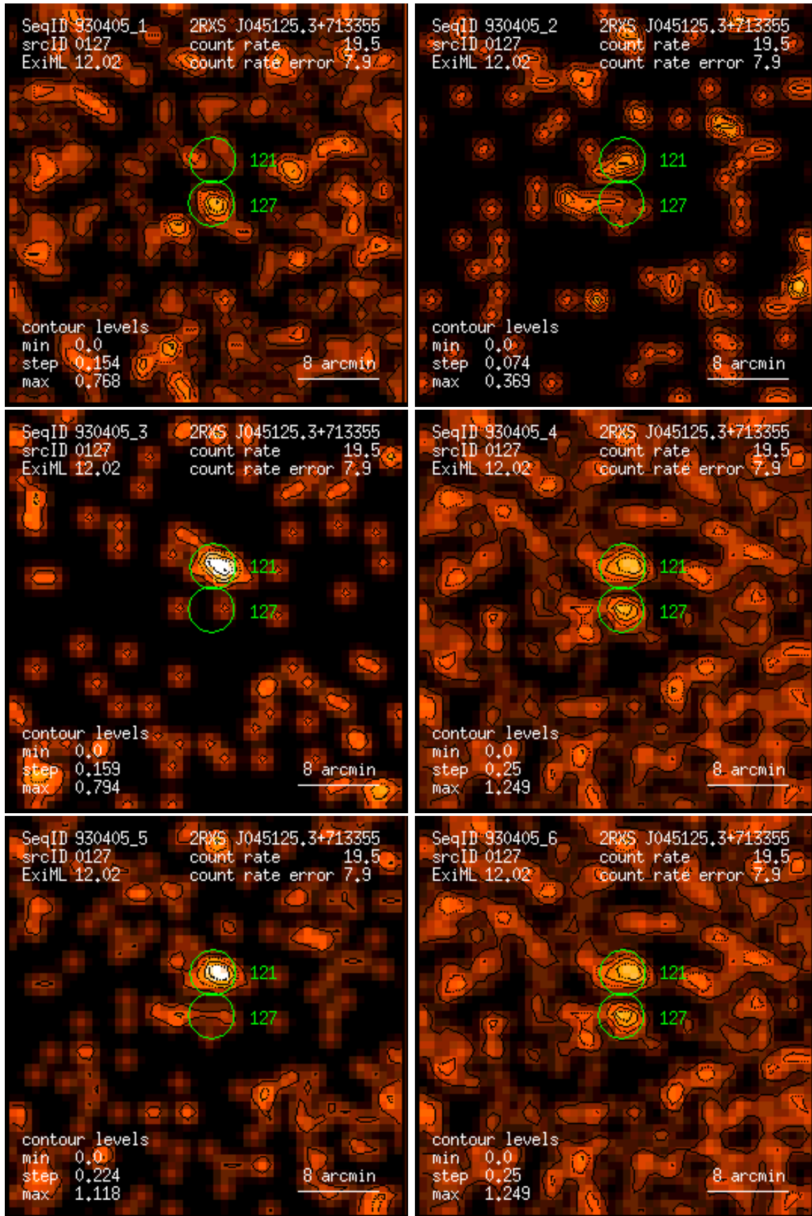
Figure 127: RASS 930405: detection 0127: band rate images, Gaussian filter: (1) PSPC channels 11 – 41, (2) 52 – 90, (3) 91 – 201, (4) 11 – 235, (5) 52 – 201, (6) 11 – 201. Broad band rates in counts/ks. Band rate contour levels in counts/ks/arcmin 2 .
