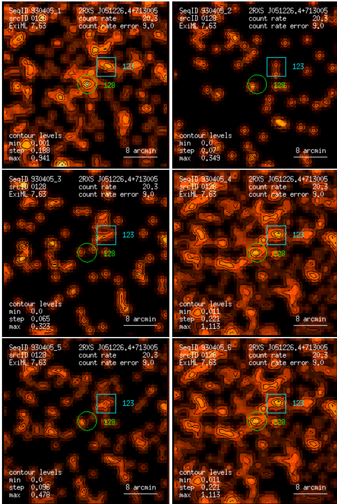
Figure 128: RASS 930405: detection 0128: band rate images, Gaussian filter: (1) PSPC channels 11 – 41, (2) 52 – 90, (3) 91 – 201, (4) 11 – 235, (5) 52 – 201, (6) 11 – 201. Broad band rates in counts/ks. Band rate contour levels in counts/ks/arcmin 2 .
