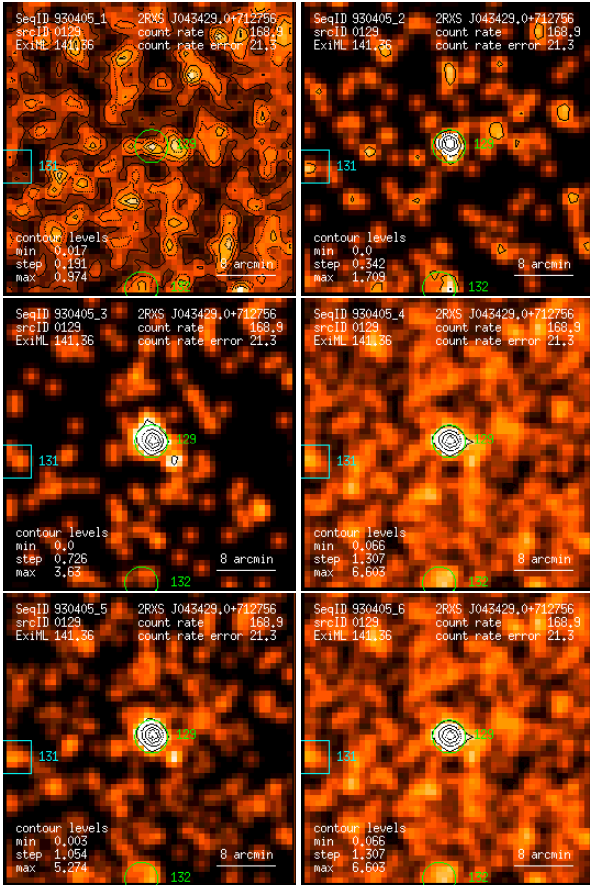
Figure 129: RASS 930405: detection 0129: band rate images, Gaussian filter: (1) PSPC channels 11 – 41, (2) 52 – 90, (3) 91 – 201, (4) 11 – 235, (5) 52 – 201, (6) 11 – 201. Broad band rates in counts/ks. Band rate contour levels in counts/ks/arcmin 2 .
