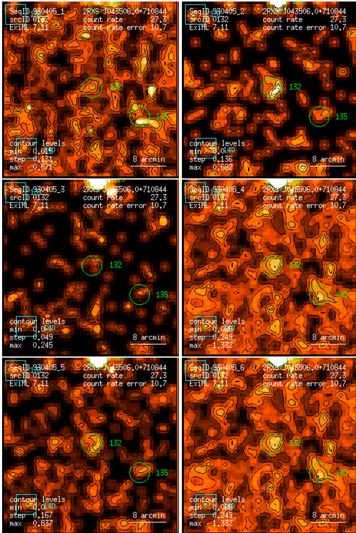
Figure 132: RASS 930405: detection 0132: band rate images, Gaussian filter: (1) PSPC channels 11 – 41, (2) 52 – 90, (3) 91 – 201, (4) 11 – 235, (5) 52 – 201, (6) 11 – 201. Broad band rates in counts/ks. Band rate contour levels in counts/ks/arcmin 2 .
