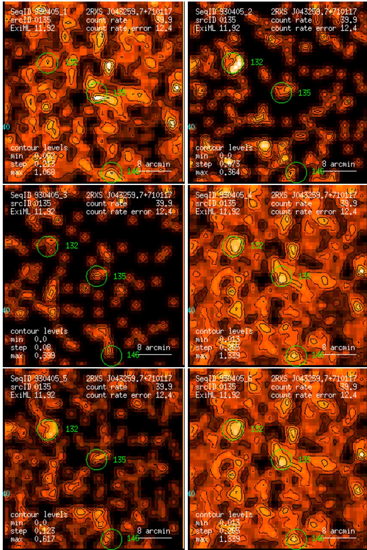
Figure 135: RASS 930405: detection 0135: band rate images, Gaussian filter: (1) PSPC channels 11 – 41, (2) 52 – 90, (3) 91 – 201, (4) 11 – 235, (5) 52 – 201, (6) 11 – 201. Broad band rates in counts/ks. Band rate contour levels in counts/ks/arcmin 2 .
