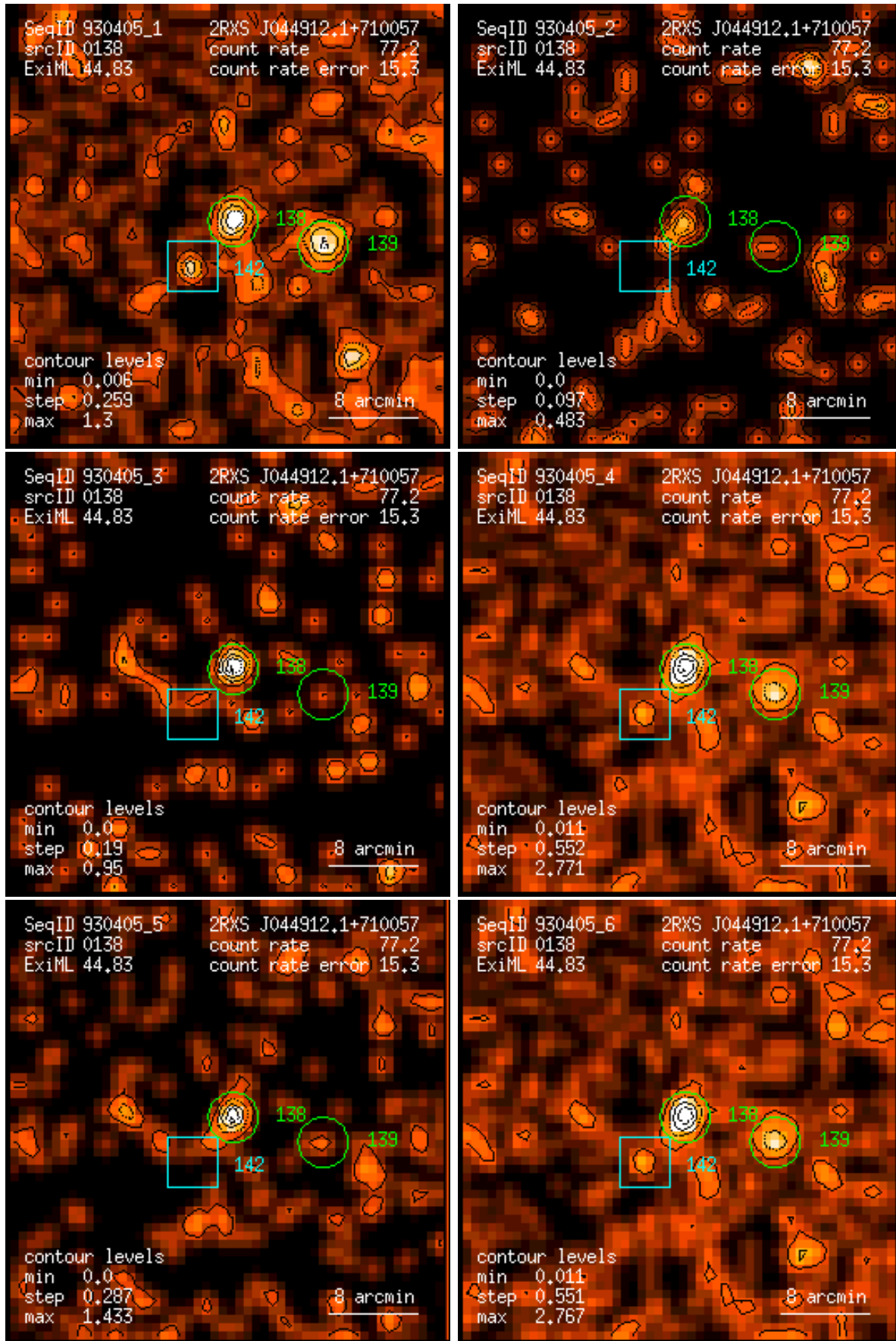
Figure 138: RASS 930405: detection 0138: band rate images, Gaussian filter: (1) PSPC channels 11 – 41, (2) 52 – 90, (3) 91 – 201, (4) 11 – 235, (5) 52 – 201, (6) 11 – 201. Broad band rates in counts/ks. Band rate contour levels in counts/ks/arcmin 2 .
