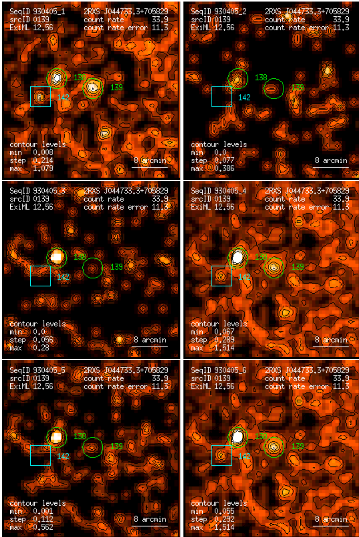
Figure 139: RASS 930405: detection 0139: band rate images, Gaussian filter: (1) PSPC channels 11 – 41, (2) 52 – 90, (3) 91 – 201, (4) 11 – 235, (5) 52 – 201, (6) 11 – 201. Broad band rates in counts/ks. Band rate contour levels in counts/ks/arcmin 2 .
