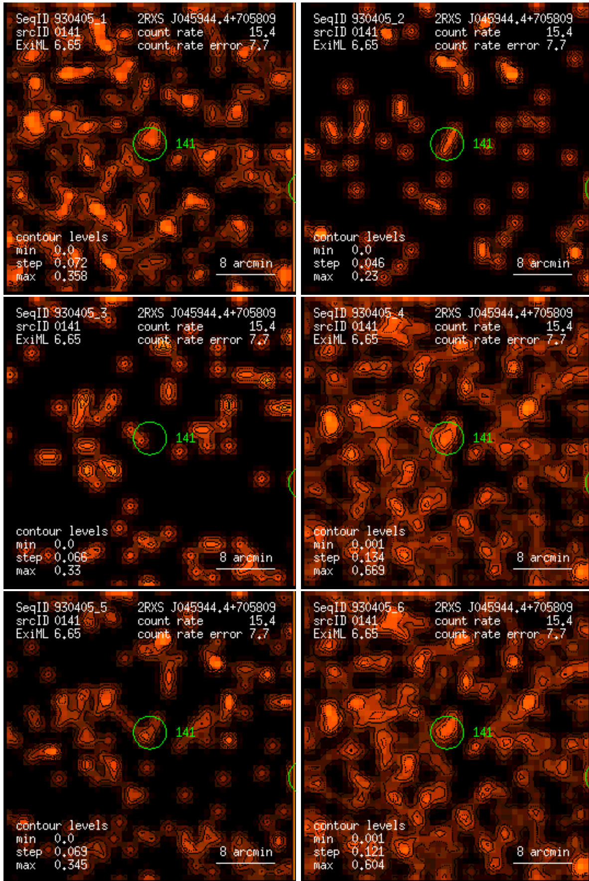
Figure 141: RASS 930405: detection 0141: band rate images, Gaussian filter: (1) PSPC channels 11 – 41, (2) 52 – 90, (3) 91 – 201, (4) 11 – 235, (5) 52 – 201, (6) 11 – 201. Broad band rates in counts/ks. Band rate contour levels in counts/ks/arcmin 2 .
