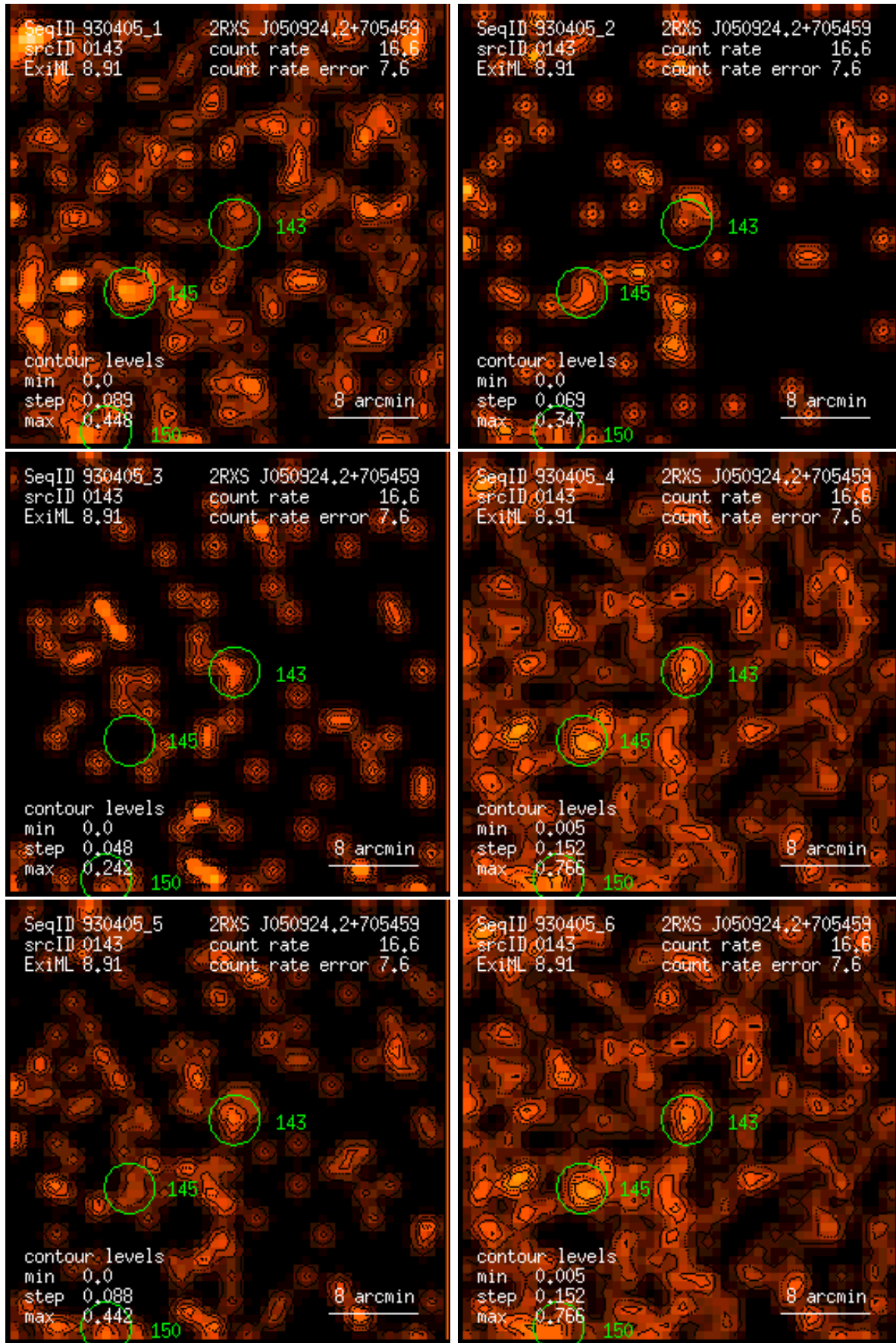
Figure 143: RASS 930405: detection 0143: band rate images, Gaussian filter: (1) PSPC channels 11 – 41, (2) 52 – 90, (3) 91 – 201, (4) 11 – 235, (5) 52 – 201, (6) 11 – 201. Broad band rates in counts/ks. Band rate contour levels in counts/ks/arcmin 2 .
