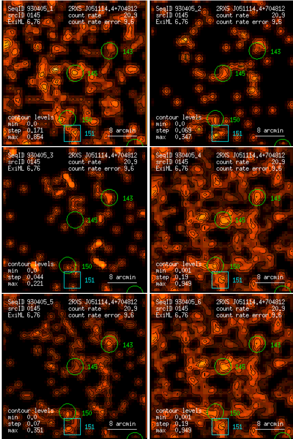
Figure 145: RASS 930405: detection 0145: band rate images, Gaussian filter: (1) PSPC channels 11 – 41, (2) 52 – 90, (3) 91 – 201, (4) 11 – 235, (5) 52 – 201, (6) 11 – 201. Broad band rates in counts/ks. Band rate contour levels in counts/ks/arcmin 2 .
