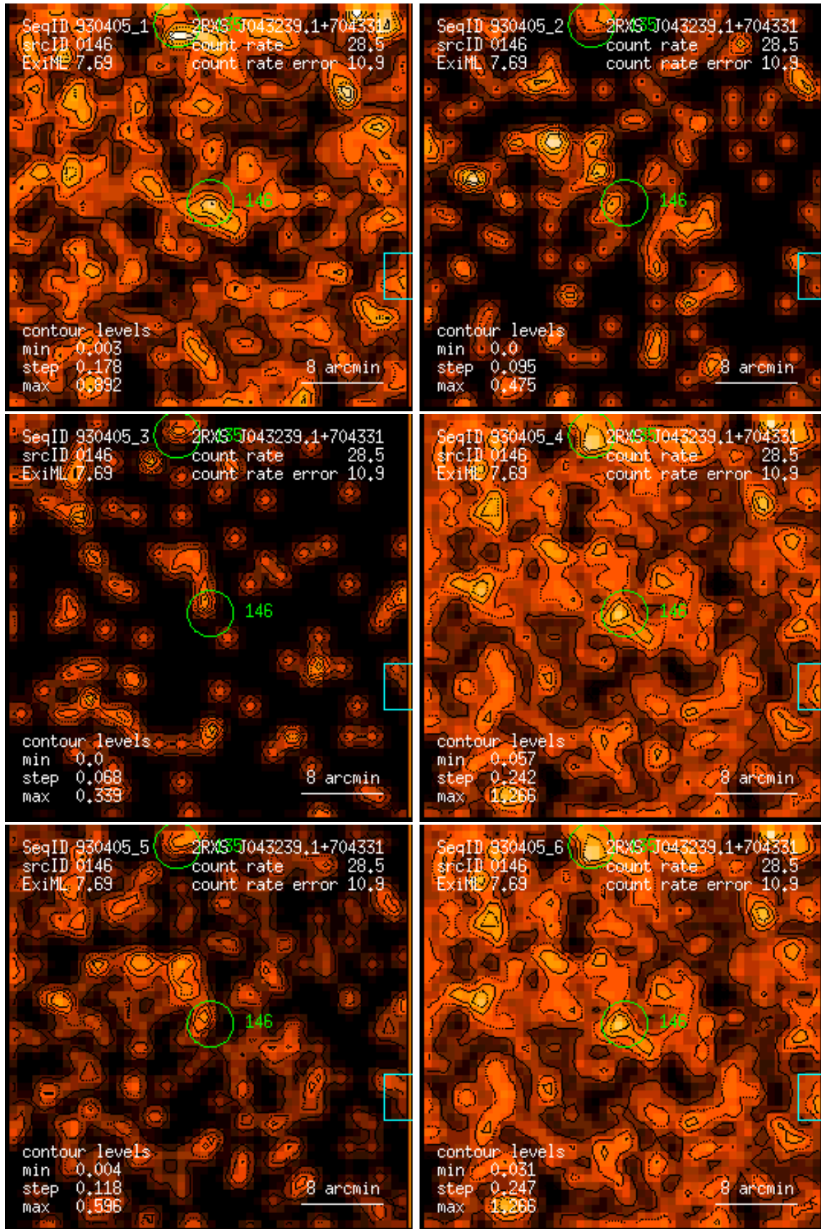
Figure 146: RASS 930405: detection 0146: band rate images, Gaussian filter: (1) PSPC channels 11 – 41, (2) 52 – 90, (3) 91 – 201, (4) 11 – 235, (5) 52 – 201, (6) 11 – 201. Broad band rates in counts/ks. Band rate contour levels in counts/ks/arcmin 2 .
