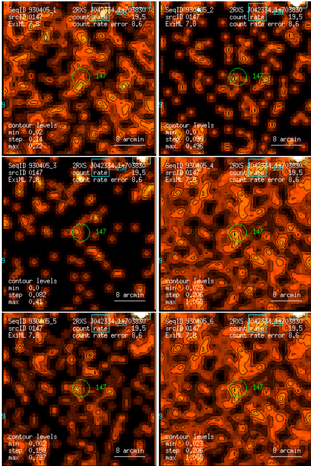
Figure 147: RASS 930405: detection 0147: band rate images, Gaussian filter: (1) PSPC channels 11 – 41, (2) 52 – 90, (3) 91 – 201, (4) 11 – 235, (5) 52 – 201, (6) 11 – 201. Broad band rates in counts/ks. Band rate contour levels in counts/ks/arcmin 2 .
